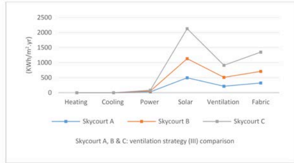
Figure 11: Annual heating, cooling, solar, fabric, ventilation and power loads comparison for skycourts (A), (B) and (C): ventilation strategies (I), (II) and (III).
